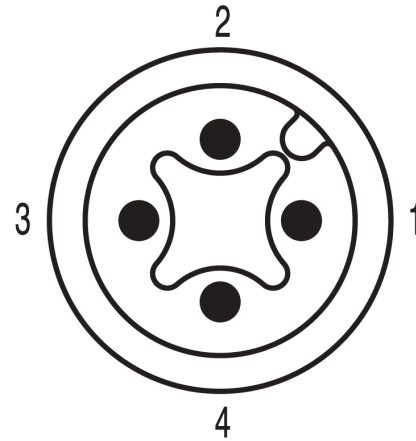
Pole scheme
