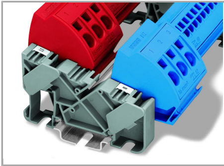
Busbar carrier (812-140):
