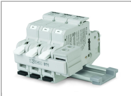
Jumper bar for quick and convenient commoning
