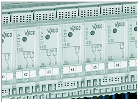
Marking using miniature WSB quick marking card
