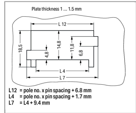
Sheet metal cutout
