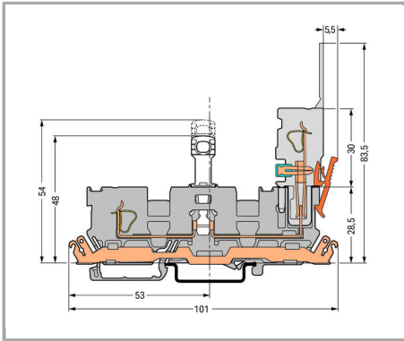
Disconnect carrier terminal block with shield contact
