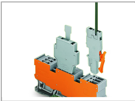
1-conductor/1-pin carrier terminal block with two jumper positions
