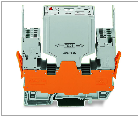
2-pin carrier terminal block for pluggable modules with orange separator plate
