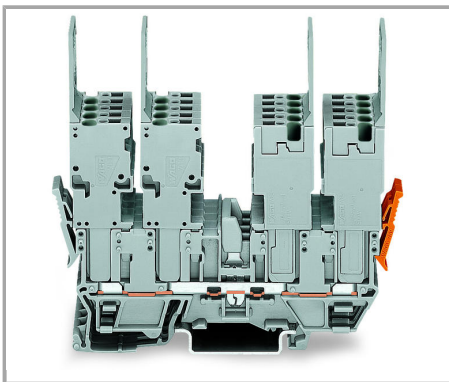
4 x 1-conductor female plugs
