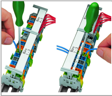
Sliding marking strips laterally.
