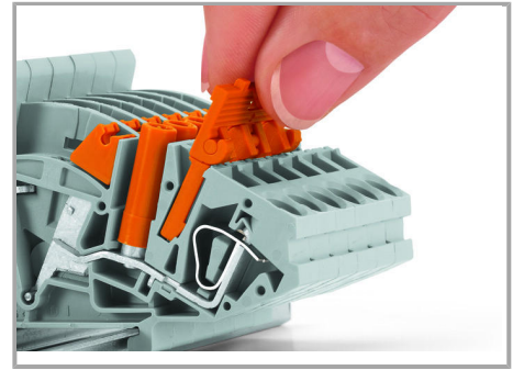
Removing a jumper via safety lid.
