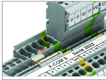
Pairing push-in comb style jumpers.
