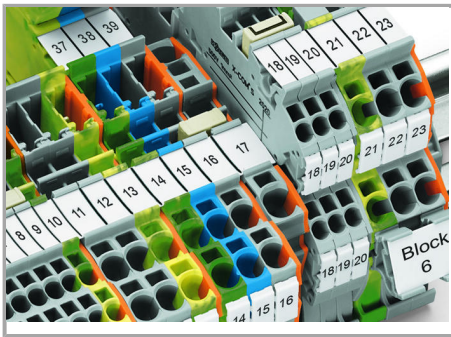
Commoning X-COM®S-SYSTEM Terminal Blocks using jumpers for TOPJOB® S Terminal Blocks. An end plate provides connection to TOPJOB® S Terminal Blocks. 2020 and 2022 Series Terminal Blocks are combinable. Jumper slots are on the same level for both series.
