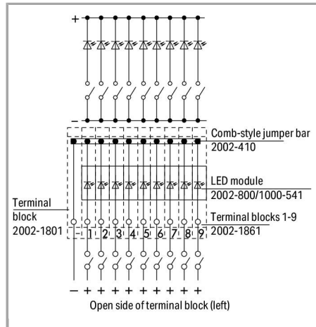
LED module (2002-800/1000-541)
