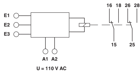
Block diagram
