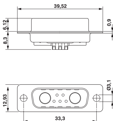
Dimensional drawing
