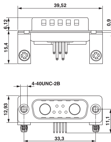
Dimensional drawing
