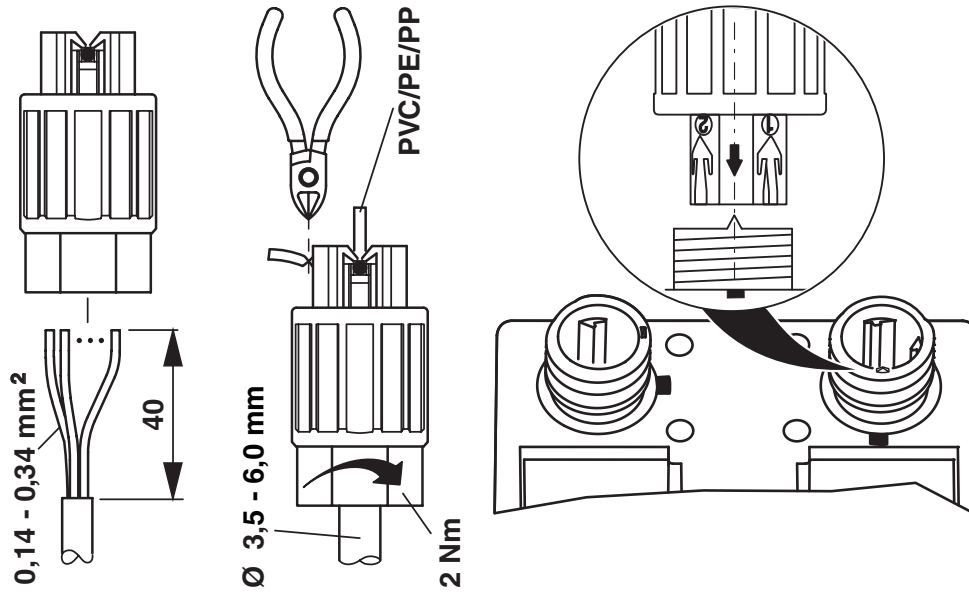
Functional drawing
