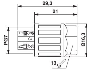
Functional drawing
