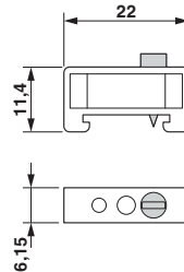
Dimensional drawing
