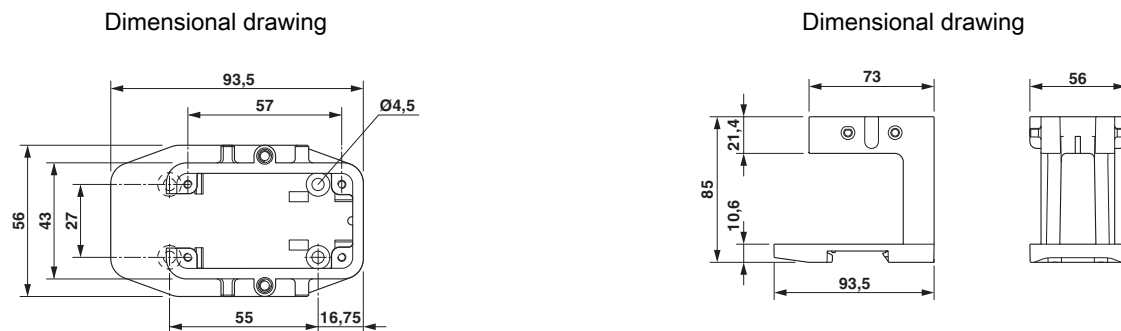
Dimensional drawing top view
