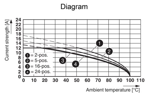
Type: MSTB 2,5/...-ST with MSTBVA 2,5/...-G
