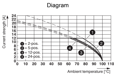
Type: MSTB 2,5/...-ST with MSTBA 2,5/...-G
