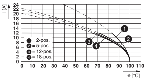
Type: MSTB 2,5/...-ST with FKIC 2,5/...-ST
