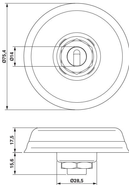
Dimensional drawing
