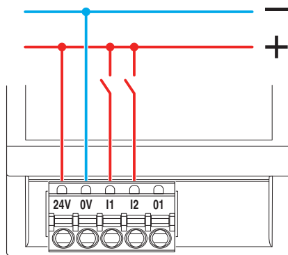
Connection diagram
