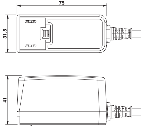
Dimensional drawing
