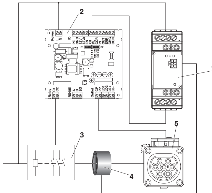
Connection diagram
