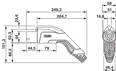
Infrastructure plug
