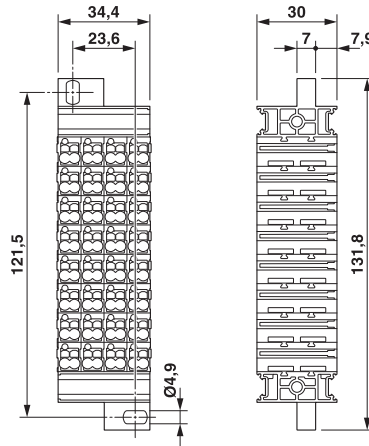
Dimensional drawing
