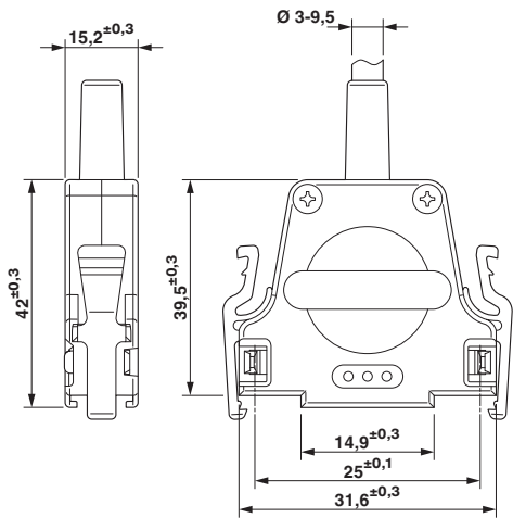
D-SUB sleeve housings
