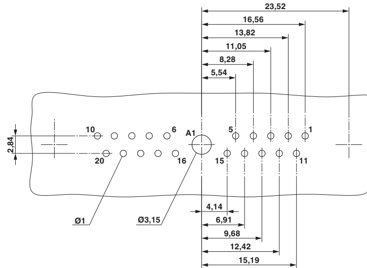
Drilling diagram
