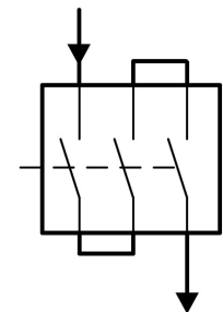
Circuit type: 1 pole, + or -, two sides
