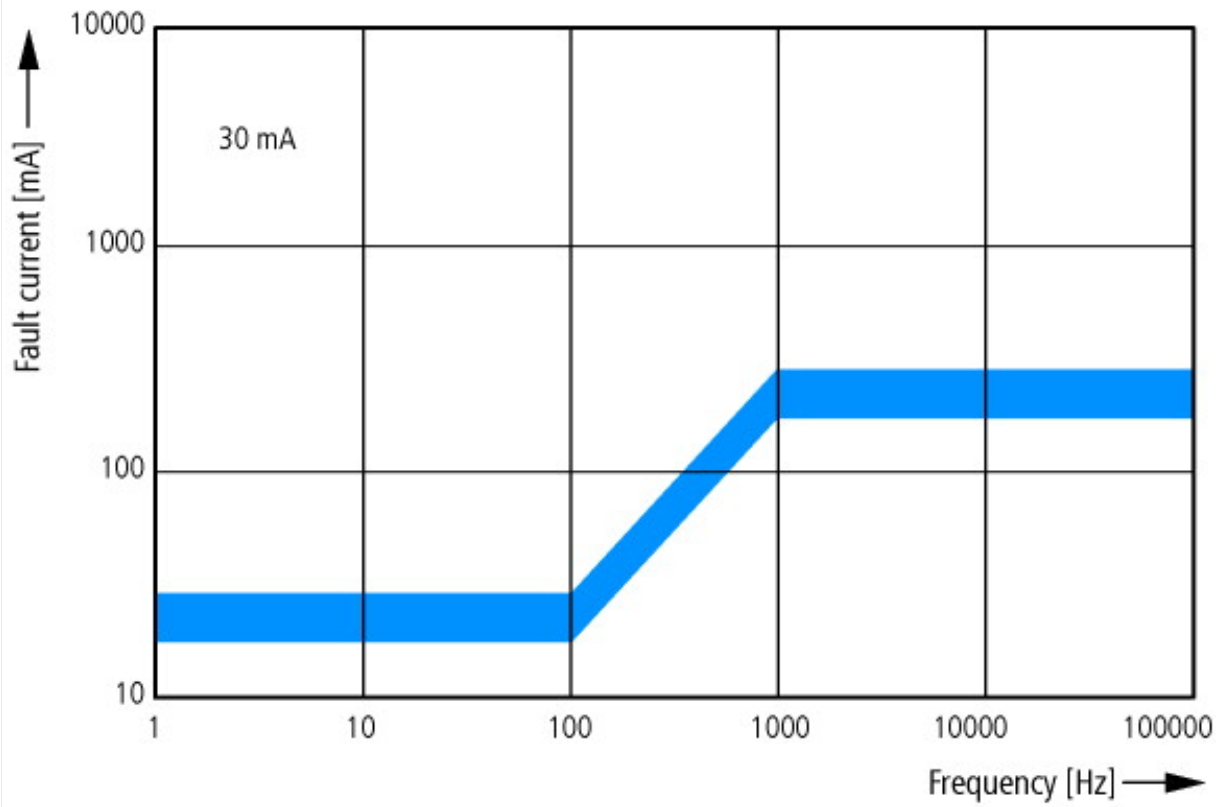
Frequency response of the tripping current 30 mA
