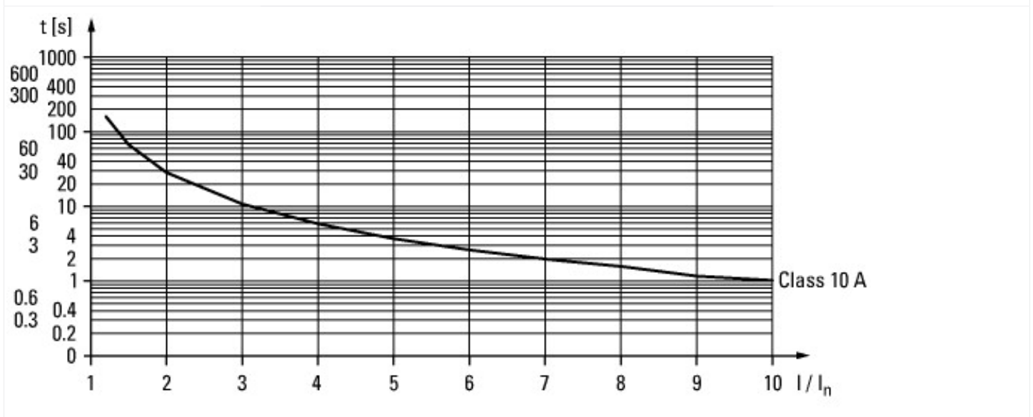
Tripping characteristics CLASS 10
