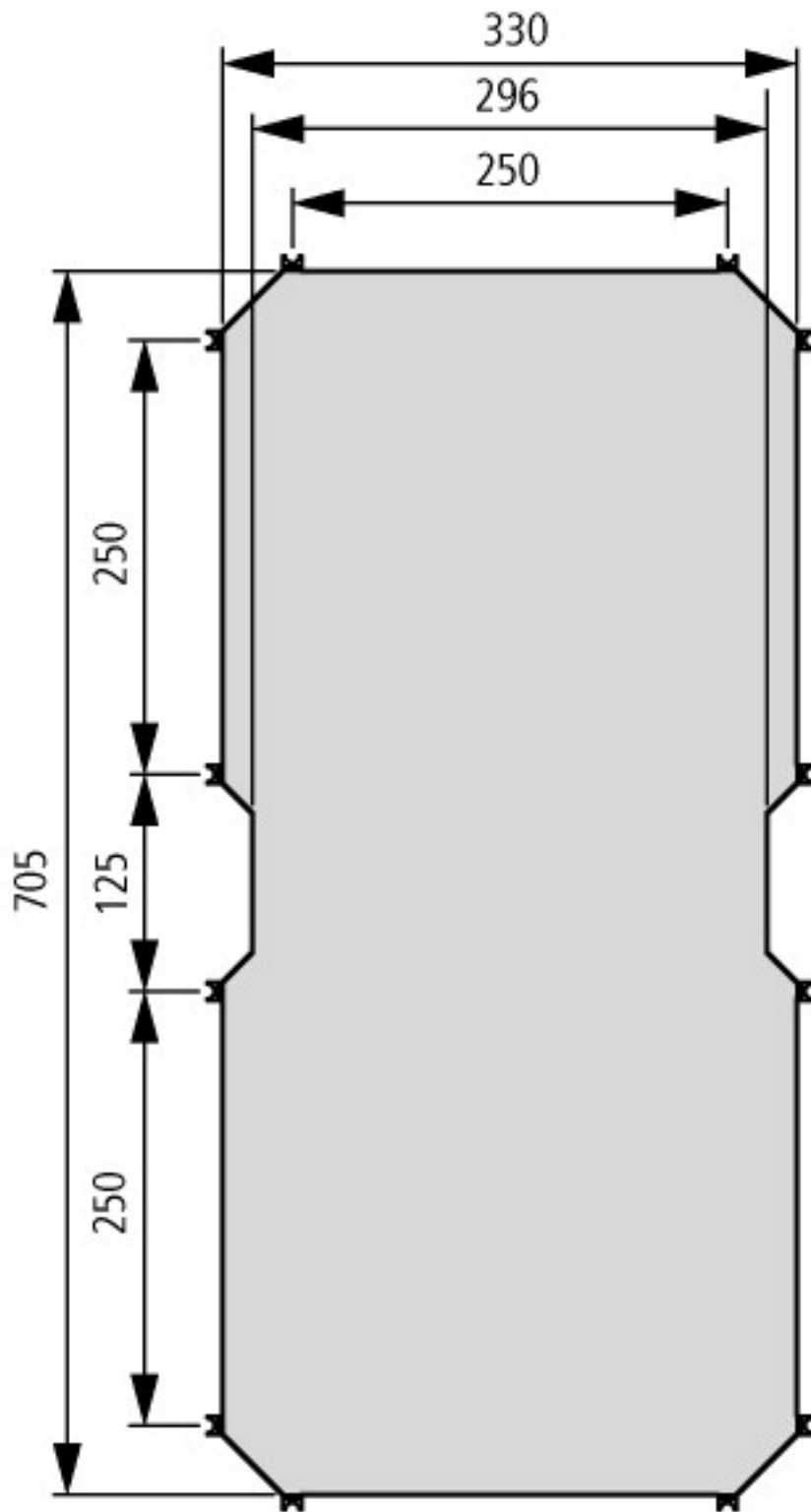
Pre-drilled mounting plate, 3 mm thick
