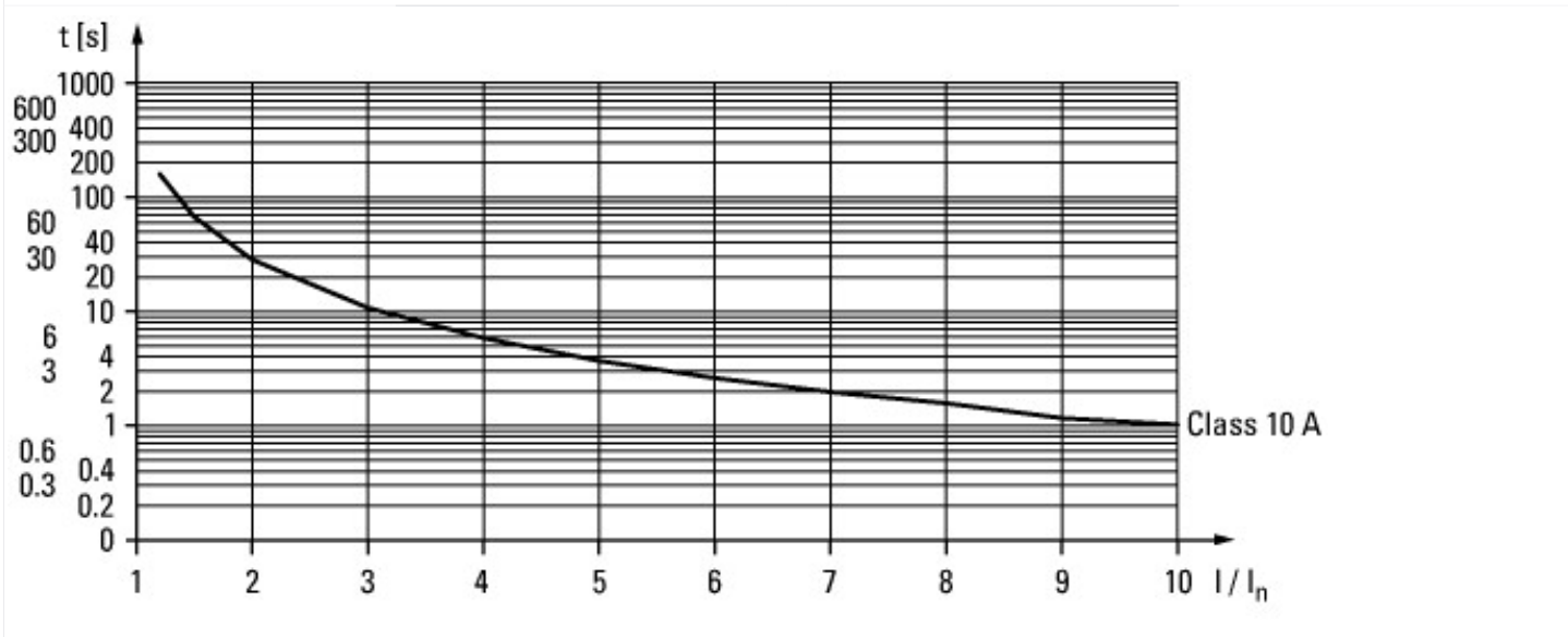
Tripping characteristics CLASS 10A
